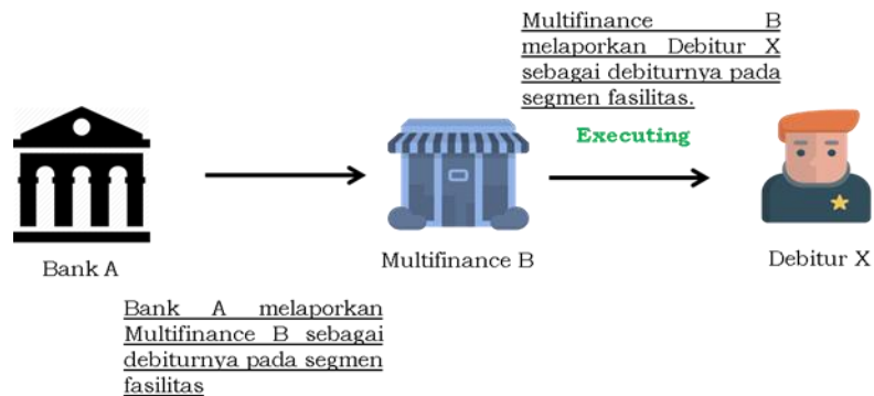
Gambar 10. Skema Executing
